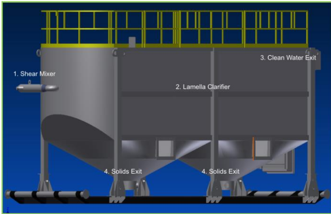
Fig. 5 - High-Volume Dewatering System Separation Module Process Flow
