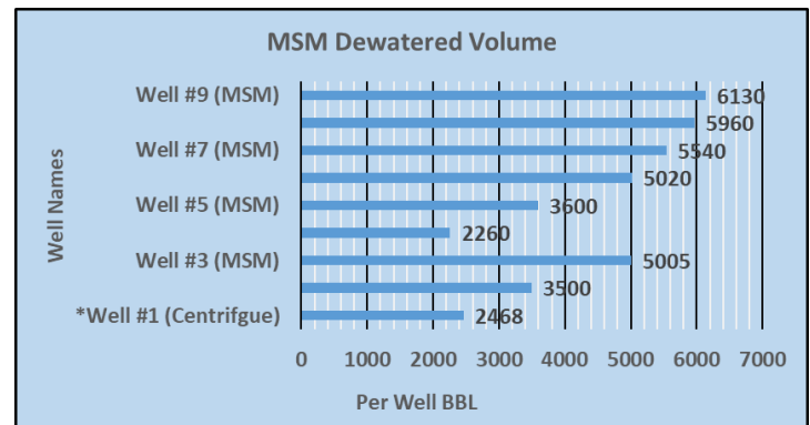
Fig. 6 – Comparison between wells & Dewatering Methods (MSM= High-Volume Dewatering System).
